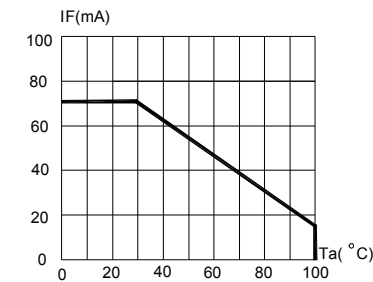
FIG.5 MAXIMUM FORWARD DC CURRENT VS AMBIENT TEMPERATURE ( T_{jmax}=120^{\circ}C )
