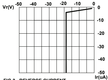
FIG.3 REVERSE CURRENT VS. REVERSE VOLTAGE.
