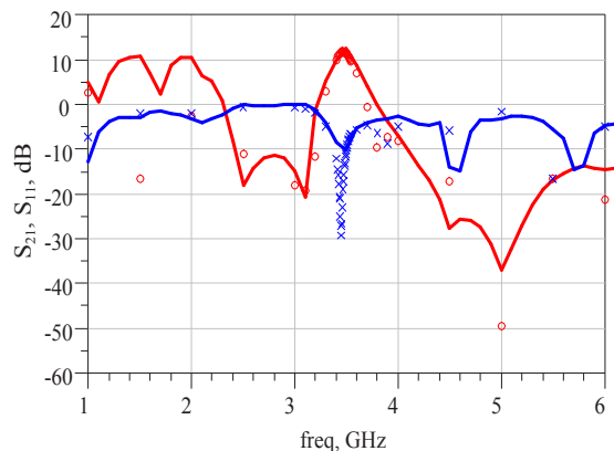
Fig. 6: Simulations (solid lines) and measurements (symbols) for S_{11} (blue) and S_{21} (red) of the DPA.
