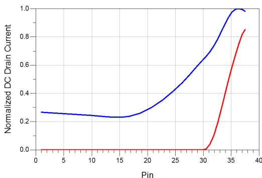
Fig. 9: Measured DC drain currents of Main (Blue) and Peak (Red) amplifiers
