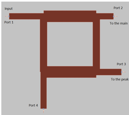
Fig. 4: Layout of the designed branch line divider.
