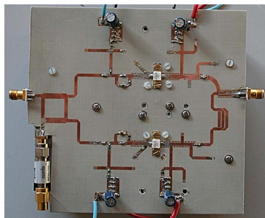
Fig. 7: Picture of the fabricated DPA.
