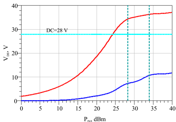
Fig. 3: Harmonic component simulation of the Main amplifier drain voltage: DC (light blue), fundamental (red) and II harmonic (blue).
