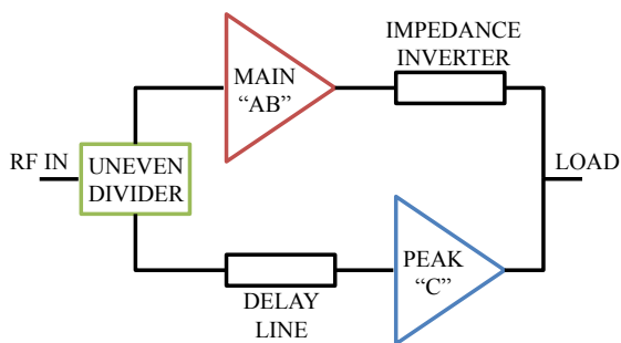
Fig. 1: Block scheme of the designed AB-C DPA.
